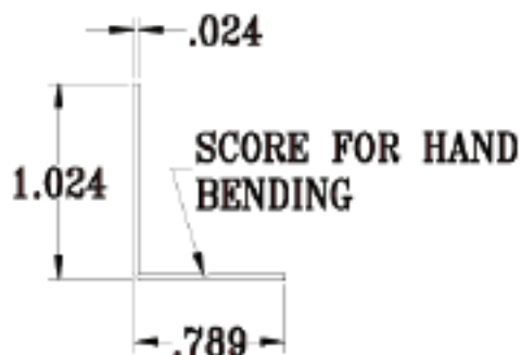
PART AS ROLL FORMED
