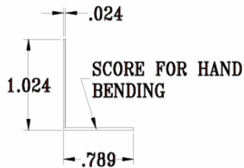
PART AS ROLL FORMED
